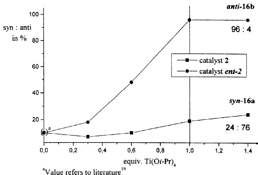
Figure 1. Diastereomeric excess of 16a,b as a function of the amount of \text{Ti}(\text{O}i\text{-Pr})_4 using either catalyst 2 or ent - 2 .
